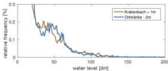
Figure 9: Statistical evaluation of water levels at Krakenbach and Orktränke . The best fit is reached applying a relative shift in elevation of 3 m, e.g., -2 m at Orktränke and +1 m at Krakenbach to show water levels relative to summer overflow at FBQ (mod. from MEYER et al., 2017).
