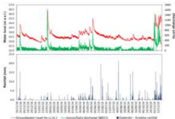
Figure 5: Comparison between water level in the Pozzo dei Frari, Isonzo river discharge (Solkán gauging station), precipitation of Doberdò Gradina (weather station).
