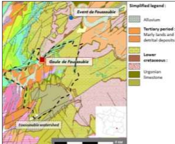
Figure 1: Localisation of the Fousoubie system. Harmonized geological map (InfoTerre, 2021 ; PASCAL et al. (1989b))
