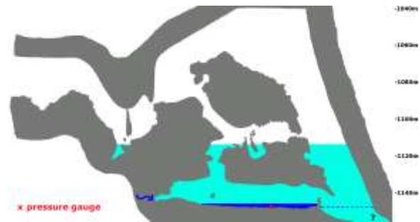
Figure 10: Cross section of Krakenkanyon near the final sump. Warm water (light blue) rising from the sump floods the passage up to 35 m above normal water level (mod. from MEYER et al., 2017).
