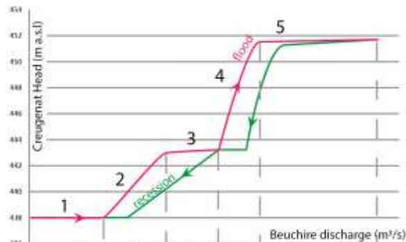
Figure 5: 1) As long as the Beuchire spring discharge rate remains lower than 700 L/s, the water level at Creugenat does not react (~438 m a.s.l.): both emergences are disconnected by a threshold. 2) As the Beuchire discharge rate exceeds 700 L/s the hydraulic head in Creugenat progressively rises up until reaching a threshold at 443 m a.s.l. This threshold may correspond to a by-pass conduit diverting the flow to the Beuchire spring, 3) as the discharge rate of the Beuchire spring increases from 1'300 L/s to 1'800 L/s the water level in Creugenat does not change (~443 m). 4) As the discharge rate exceeds 1'800 L/s the water level in Creugenat rises up again until reaching the outlet elevation at 451 m a.s.l. 5) As the discharge rate exceeds 2'200 L/s, the Creugenat spring starts overflowing.
