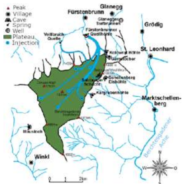
Figure 1: Dye tracing at Untersberg.
